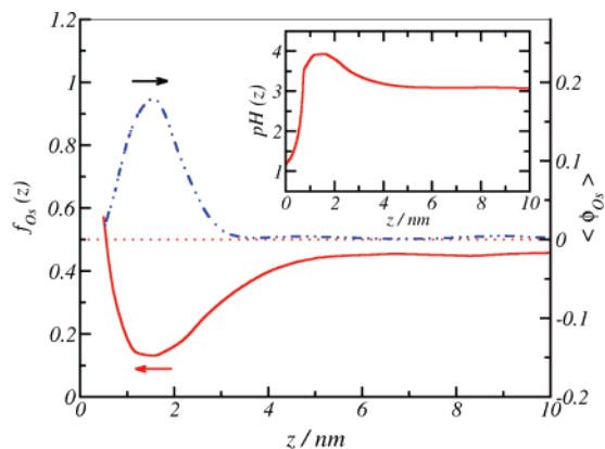
Figure 8. Fraction of oxidized redox sites (solid line, left axis) and osmium site volume fraction (dashed line, right axis) as a function of the distance from the electrode at E = E_{\text{Os(II)/Os(III)}}^0 . Inset: local pH vs distance from the electrode. The PAH-Os molecular model and the conditions of Figure 5 were used in the calculations.
