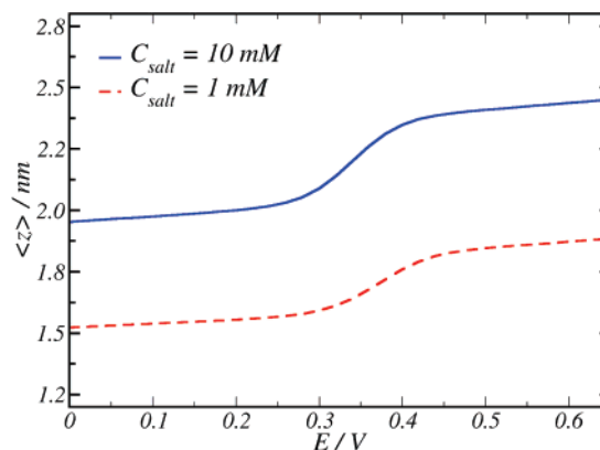
Figure 9. Theoretical predicted thickness-potential curves calculated for two different salt concentrations at pH = 3.
