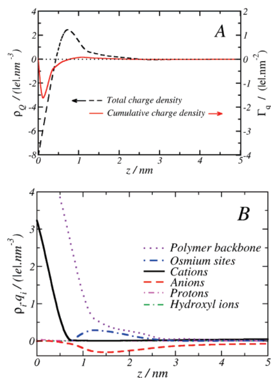
Figure 7. A. Total charge density (dashed line, left axis), eq 15, and cumulative charge density (full line, right axis), eq 47, as a function of the distance from the electrode. B. Charge density profile for each of the charged molecular species considered by the theory. The calculations were performed using the PAH-Os Molecular Model for the conditions of Figure 5. For a better visualization of the densities of protons see the inset in Figure 8.
