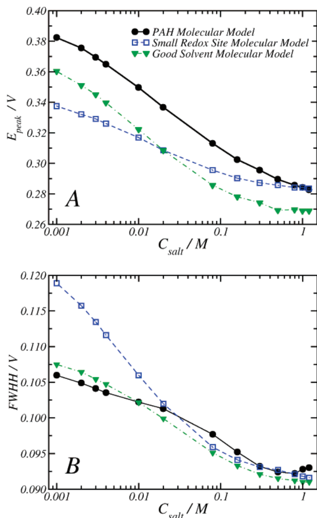
Figure 4. Plots of peak potential position (A) and peak width (B) vs salt concentration in the bulk solution calculated for different molecular models described in section 4.2 using pH = 3.
