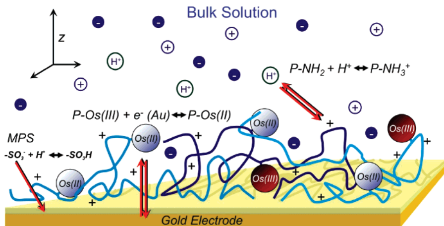
Figure 1. Schematic representation of the Au/MPS/PAH-Os/solution interface. The red arrows indicate the chemical equilibria considered by the theory. The redox polymer, PAH-Os (see Chart 1), is divided into the poly(allyl-amine) backbone (depicted as blue and light blue solid lines) and the pyridine-bipyridine osmium complexes. Each osmium complex is in redox equilibrium with the gold substrate and, depending on its potential, can be in an oxidized Os(III) (red spheres) or in a reduced Os(II) (blue sphere) state. The allyl-amine units can be in a positively charged protonated state (plus signs on the polymer backbone lines) or in a neutral deprotonated state, which are related by an acid–base equilibrium. The self-assembled layer of a mercapto-propane sulfonate, MPS, is covalently adsorbed on top of the gold substrate (depicted as a yellow layer covering the electrode). The sulfonate groups in MPS are in acid–base equilibrium with protons in solution and thus could be in a protonated or in a deprotonated state. The polymer-modified electrode is immersed in an aqueous electrolyte solution containing salt ions, protons, and hydroxyls in thermodynamic equilibrium which a bulk solution. The normal direction from the electrode is denoted by z and has its origin on the metal surface.
