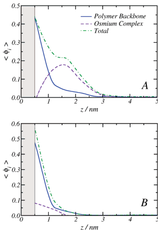
Figure 5. Theoretical volume fraction profiles for the polymer backbone (full line), the redox sites (dashed line), and the whole redox polymer (dot-dashed line) obtained for the PAH-Os molecular model described in section 3 (A), and the small redox site molecular model described in section 4.2 (B). The calculations were performed at E = E_{\text{Os(II)/Os(III)}}^0 using C_{\text{salt}} = 0.1 M and pH = 3. The shaded region ( z < 0.5 nm) is occupied by the thiol layer.
