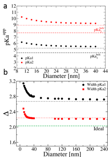
Figure 6. (a) pK_a^{\text{app}} as a function of cylindrical nanochannel diameter, D . The pK_a^{\text{app}} is defined as the pH value where \langle f_0 \rangle = \langle f_{-1} \rangle , and the pK_a^{\text{app}} is defined as the pH value where \langle f_{-1} \rangle = \langle f_{-2} \rangle . (b) Width of the transition ( \Delta ) as a function of D . The width \Delta is defined as the difference between the pH values where the degree of dissociation reaches the values of 1/11 and 10/11 ( \Delta_1 for \langle f_{-1} \rangle and \Delta_2 for \langle f_{-2} \rangle ); see text. Horizontal dashed lines show the bulk values for the pK_a 's and \Delta . Horizontal dotted lines show the predictions of the simple analytical model, eqs 20–23. Parameters: N_p/A(R) = 0.2 chains/nm 2 , degree of polymerization N = 28 , pK_{a1}^{\text{bulk}} = 4.5 , pK_{a2}^{\text{bulk}} = 7.7 , and C_{\text{salt}} = 0.1 M.
