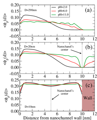
Figure 5. Polymer volume fraction \langle\phi_p(d)\rangle as a function of distance from the wall of the nanochannel, d . The curves correspond to pH = 2 (black), pH = 6.0 (red), and pH = 11 (green). The diameters of the channel are (a) D = 290 nm, (b) 20 nm, and (c) 10 nm. Other parameters: N = 28 units per chain, N_p/A(R) = 0.2 chains/nm 2 , C_{\text{salt}} = 0.1 M.
