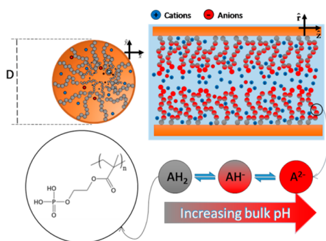
Figure 1. Scheme of a section of cylindrical nanochannel modified by an end-grafted layer of the weak polyacid (poly(2-(methacryloyloxy)-ethyl-phosphate)), PMEP. The solution inside the nanochannel contains water molecules, salt anions (small red circles), salt cations (small blue circles), hydroxyl ions, and protons. Each monomer in PMEP can exist in one of three possible chemical states: \text{PMEPH}_2 ( \text{AH}_2 ), \text{PMEPH}^- ( \text{AH}^- ), and \text{PMEP}^{2-} ( \text{A}^{2-} ).
