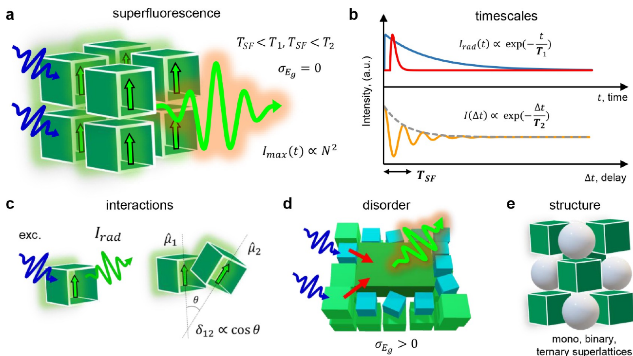
Figure 16. Superfluorescence in NC assemblies. (a) Collective superfluorescence is achieved when NC properties fulfill criteria for identical and coherent emitters. (b–e) Relevant degrees of freedom for superfluorescence. (b) Timescales of radiative decay, T_1 , first-order coherence, T_2 , and accelerated decay, T_{SF} , are of correct relative order to favor superfluorescence, for example, T_{SF} < T_1 , T_{SF} < T_2 . (c) Coupling of dipole-dipole interactions between close-packed NCs contributes to radiative coupling, where \hat{\mu}_1 and \hat{\mu}_2 are unit vectors of transition electric dipole, and \delta_{12} is the orientation-dependent interaction energy. (d) Disorder leading to energetic inhomogeneity shall be minimized as it leads to excitation localization as opposed to the collective state. For example, size dispersion results in the energy transfer between NCs with different E_g . (e) Mixing NC building blocks is a strategy to tune cooperative emission.
