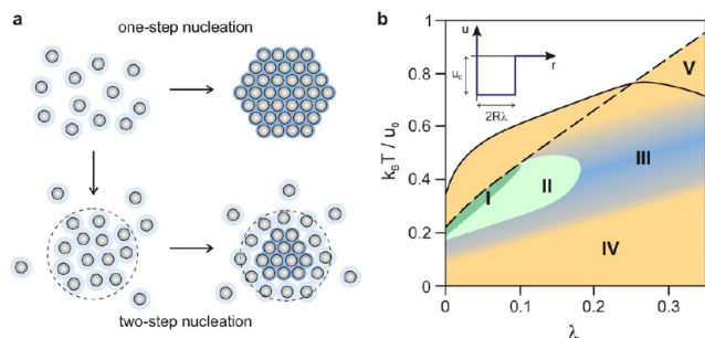
Figure 11. Nucleation of NC assemblies. (a) Schematic representation of one-step and two-step nucleation processes. (b) Probability of superlattice nucleation represented by color gradients, where green is high, blue is intermediate, and yellow is a low probability. The axes represent the depth u_0 and range \lambda of a square-well potential, as represented in the inset, for colloidal particles with radius R and a volume fraction of 0.1. The diagram shows the regions of (I) one-step nucleation, (II) two-step nucleation, (III) the coexistence of two metastable fluids with a slow nucleation rate, (IV) gel formation, and (V) a thermodynamically stable colloidal fluid. The dashed line is the metastable fluid-fluid binodal curve. The solid black curve is the thermodynamic boundary for the stability of an fcc crystal. Adapted with permission from ref 27. Copyright 2022 The American Association for the Advancement of Science. Based on data of ref 21.
