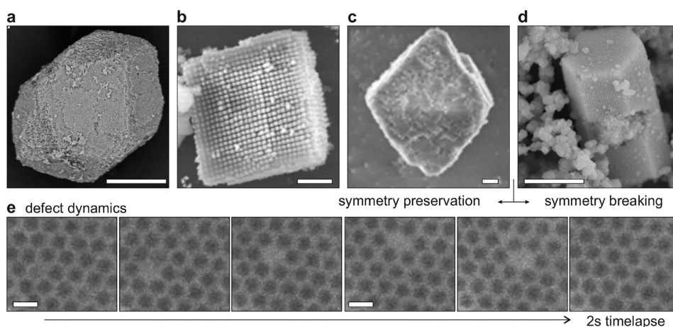
Figure 12. Microscopy of superstructures formed of NCs. (a–d) Scanning electron microscopy of superhabits formed by the assembly of DNA-functionalized NCs. Superhabits can preserve the symmetry of the superlattice, forming (a) rhombic dodecahedra, 28 (b) cubes, 526 and (c) and octahedra; 526 or break symmetry as shown in (d) via the formation of energetic barriers in certain crystalline directions due to plane multiplicity of the AB_2 superlattice formed by an NC alloy. 29 (e) Liquid cell TEM showing a vacancy diffusion in a superstructure, evidencing the dynamics of superstructure defects. 457 Scale bars, 1 \mu\text{m} (a–d) and 100 nm (e). (a) Reprinted in part with permission from ref 28. Copyright 2014 Springer Nature BV. (b, c) Reprinted in part with permission under a Creative Commons CC BY license from ref 526. Copyright 2016 American Chemical Society. (d) Adapted with permission under a Creative Commons CC BY license from ref 29. Copyright 2018 Springer Nature. (e) Reprinted in part with permission from ref 457. Copyright 2022 American Chemical Society.
