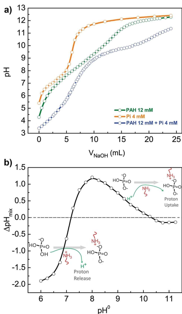
Figure 4. System pH response without added KCl. a) Potentiometric titration curves of 40 mL PAH 12 mM (green line), 40 mL NaH 2 PO 4 4 mM (orange line), 40 mL PAH 12 mM + NaH 2 PO 4 4 mM (blue line). The solutions were titrated with 30 mM NaOH. b) Shift of the pH due to the mixing process vs. initial pH.
