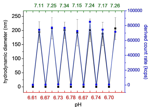
Figure 8. Dynamic light scattering hydrodynamic diameter and derived count rate of PAH/Pi crosslinked nanostructures in aqueous solution in presence of 0.2 M KCl at different consecutive pH. Colloid formation/dissolution reversibility near physiological pH.
