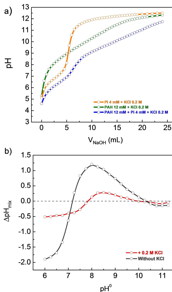
Figure 7. System pH response with added KCl. a) Potentiometric titration curves of 40 mL 12 mM PAH + 0.2 M KCl (green line), 40 mL 4 mM \text{NaH}_2\text{PO}_4 + 0.2 M KCl (orange line) and 40 mL 12 mM PAH + 4 mM \text{NaH}_2\text{PO}_4 + 0.2 M KCl (blue line) with 30 mM NaOH. b) Shift on the pH by the mixing process vs initial pH. For comparison, the system without added KCl is also shown (grey line).
