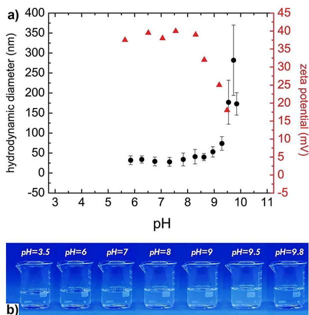
Figure 1. Colloid pH stability window without added KCl. a) Hydrodynamic diameter (black circles) and Zeta potential (red triangles) vs. solution pH for the titration of 40 mL PAH 12 mM + \text{NaH}_2\text{PO}_4 4 mM with NaOH 30 mM. b) Photographs of the solution for increasing pHs.
