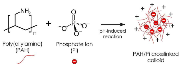
Scheme 1. Simplified PAH/Pi crosslinked colloid formation scheme.
