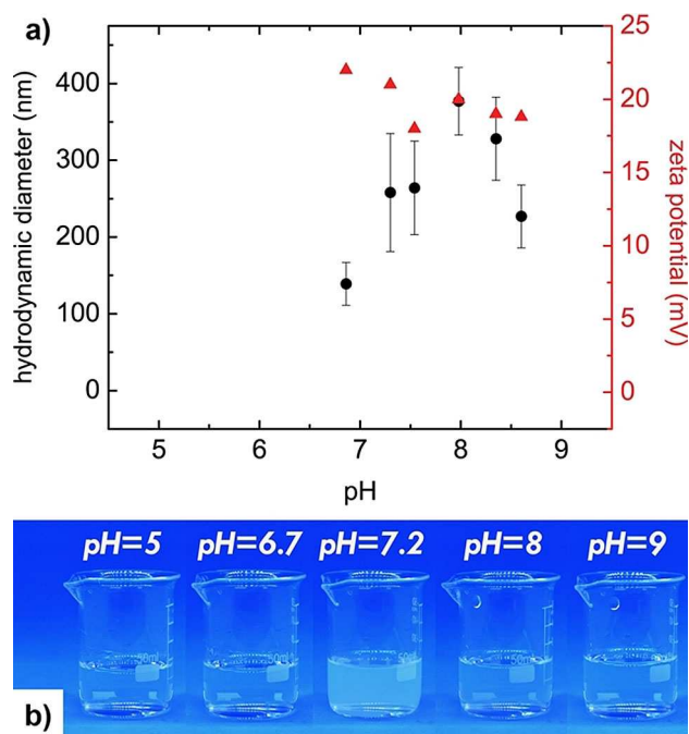
Figure 6. Colloid pH stability window with added KCl. a) Hydrodynamic diameter (black circles) and Zeta potential (red triangles) vs solution pH of 40 mL PAH 12 mM + \text{NaH}_2\text{PO}_4 4 mM + 0.2 M KCl titrated with NaOH 30 mM. b) Photographs indicating the solution fashion with increasing pH.
