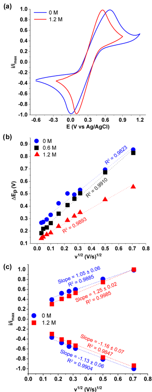
Figure 5. (a) Cyclic voltammograms recorded at 250 mV/s for PEI/ \text{Fe}(\text{CN})_6^{3-} coacervates formed in the presence of NaCl 0 or 1.2 M. (b) Separation of the anodic and cathodic peak potentials versus the square root of scan rate, v^{1/2} , measured for coacervates prepared with different concentrations of added NaCl. (c) Peak currents for the anodic ( i/i_{\max} > 0 ) and cathodic ( i/i_{\max} < 0 ) vs v^{1/2} measured for coacervates formed in the presence of NaCl 0 M or 1.2 M versus the scan rate. The currents are normalized by i_{\max} , which is the peak current determined for v^{1/2} = 0.707 (V/s) 1/2 (0.5 V/s).
