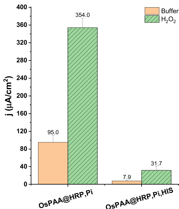
Fig. 7. Current densities for cyclic voltammetries carried out at 10 \text{ mV s}^{-1} performed in 50 mM acetate buffer + 0.15 M NaCl, pH 5.0 (filled) and in the presence of 2 mM \text{H}_2\text{O}_2 in the same buffer (black lines) for different matrices with HRP.
