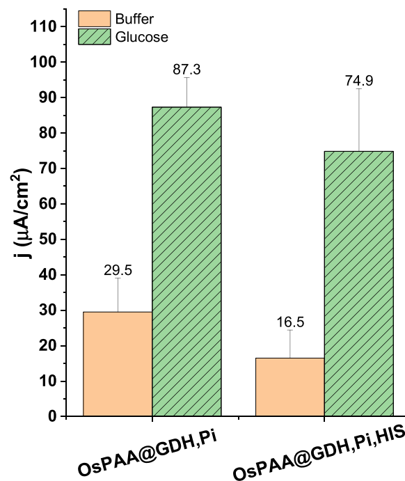
Fig. 6. Current densities for cyclic voltammeteries carried out at 10 mV s -1 performed in 50 mM HEPES buffer + 0.1 M NaCl, pH 7.0 (filled) and in the presence of 100 mM Glucose in the same buffer (black lines) for different matrices with GDH.
