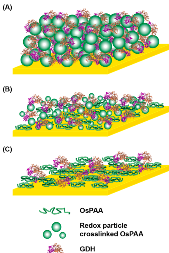
Scheme 2. Description of modified surfaces via LbL self-assembly process using GDH and OsPAA as (A) unimodal redox particles in @Pi matrix, (B) bimodal smaller redox particles in @Pi, HIS matrix and (C) random-coil in @H 2 O.
